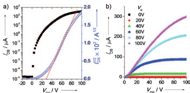
Figure 3. I – V characteristics of Cl 8 -PTCDI TFT prepared on OTS-treated SiO 2 /Si at T D = 125 °C. a) Plot of I_{DS} vs. V_{GS} for V_{DS} = 100 V. b) Plot of I_{DS} vs. V_{DS} . The measurement was carried out under nitrogen atmosphere.
